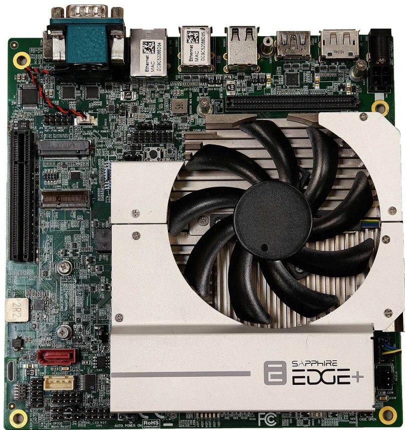
Mainboard with Cooler picture
